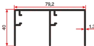
LG 329 0.759 Kg/mt
