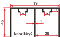
LG 328 0.655 Kg/mt
