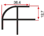
LG 250 0.462 Kg/mt
