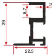
LG 419 A 0.421 Kg/mt
